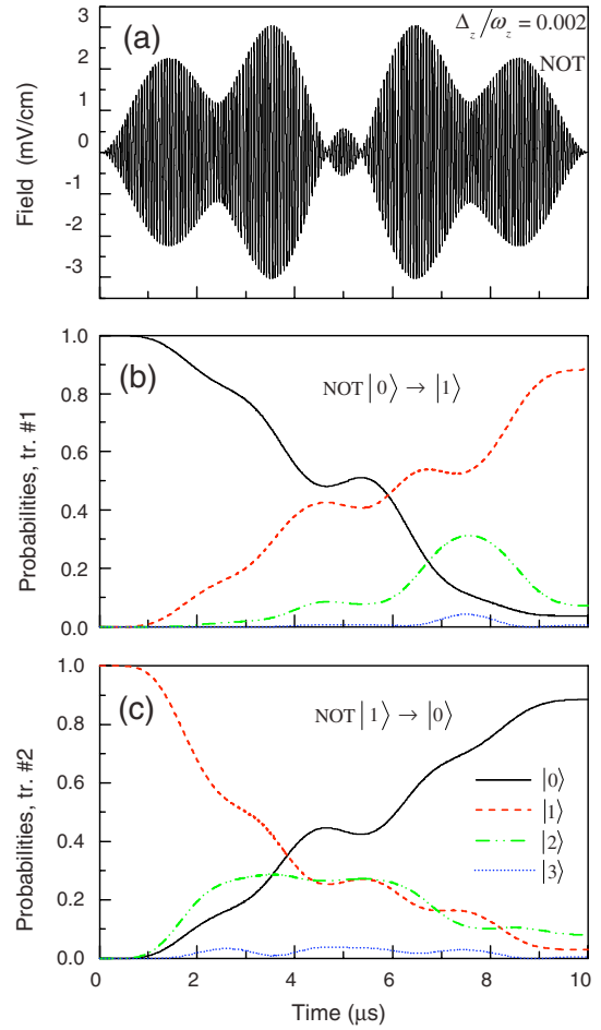
FIG. 3. (Color online) Same as in Fig. 1 but for \Delta_z/2\pi=5.54 kHz (an insufficient anharmonicity case).
