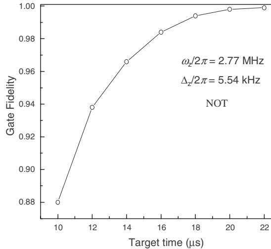
FIG. 4. Fidelity of the gate NOT as a function of pulse duration T for the anharmonicity parameter \Delta_z/2\pi=5.54 kHz.
