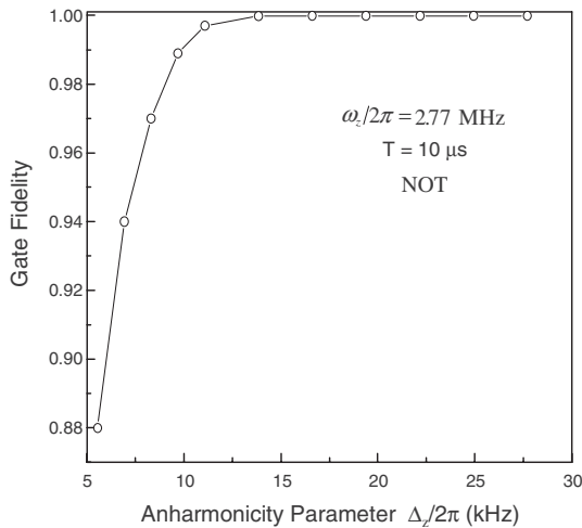
FIG. 2. Fidelity of the gate NOT as a function of anharmonicity parameter for the \text{Cd}^+ ion trap with \omega_z/2\pi=2.77 MHz. The target time is T=10 \mu\text{s} .
