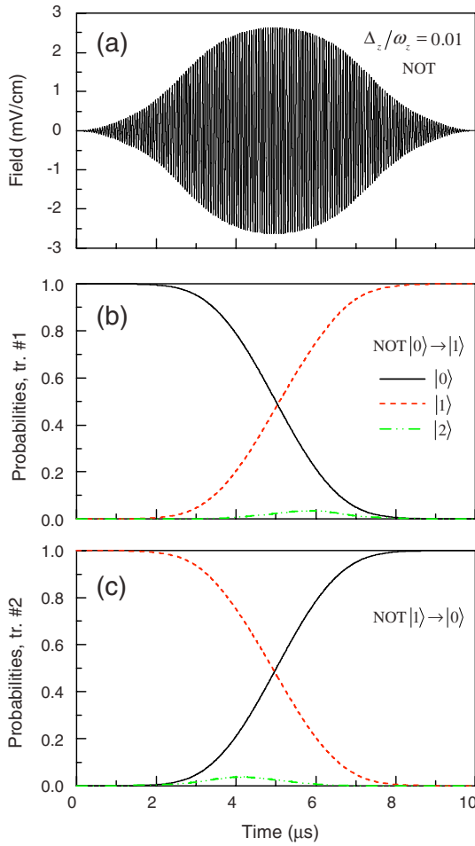
FIG. 1. (Color online) The gate NOT in the \text{Cd}^+ ion trap with \omega_z/2\pi=2.77 MHz and the anharmonicity parameter \Delta_z/2\pi=27.7 kHz: (a) optimally shaped electric field; (b) switching of population between the qubit states during the NOT |0\rangle\rightarrow|1\rangle transformation; (c) the same during the NOT |1\rangle\rightarrow|0\rangle transformation.
