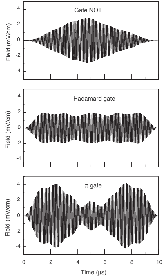
FIG. 5. A set of universal one-qubit gates for \Delta_z/2\pi = 15.5 kHz. The target time is T=10 \mu\text{s} .
